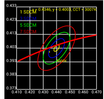
IEC SDCM Diagram
