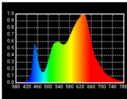
Typical spectral and colorimetric performance at 3000K
