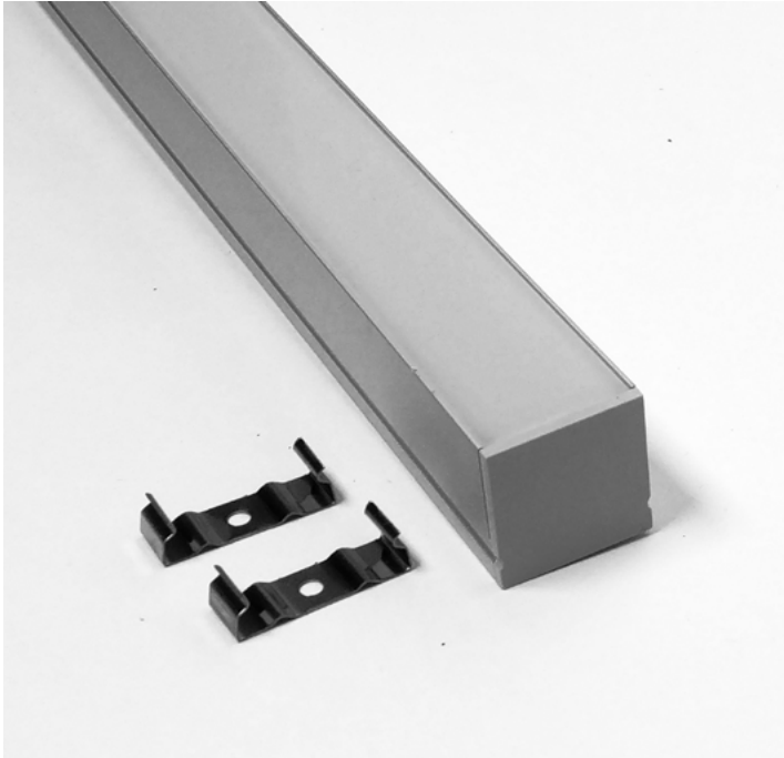
2525 aluminum surface-mount LED profile (can accept single LED strip up to 20mm wide, or two 10mm wide LED strips)
