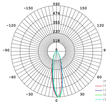
AVERAGE BEAM ANGLE (50%): 25.1 DEG
