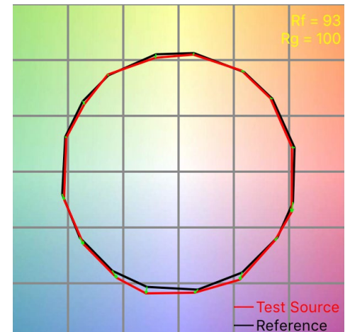
TM-30-15 Diagram
